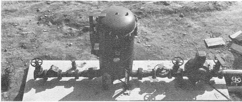
Filter separator
