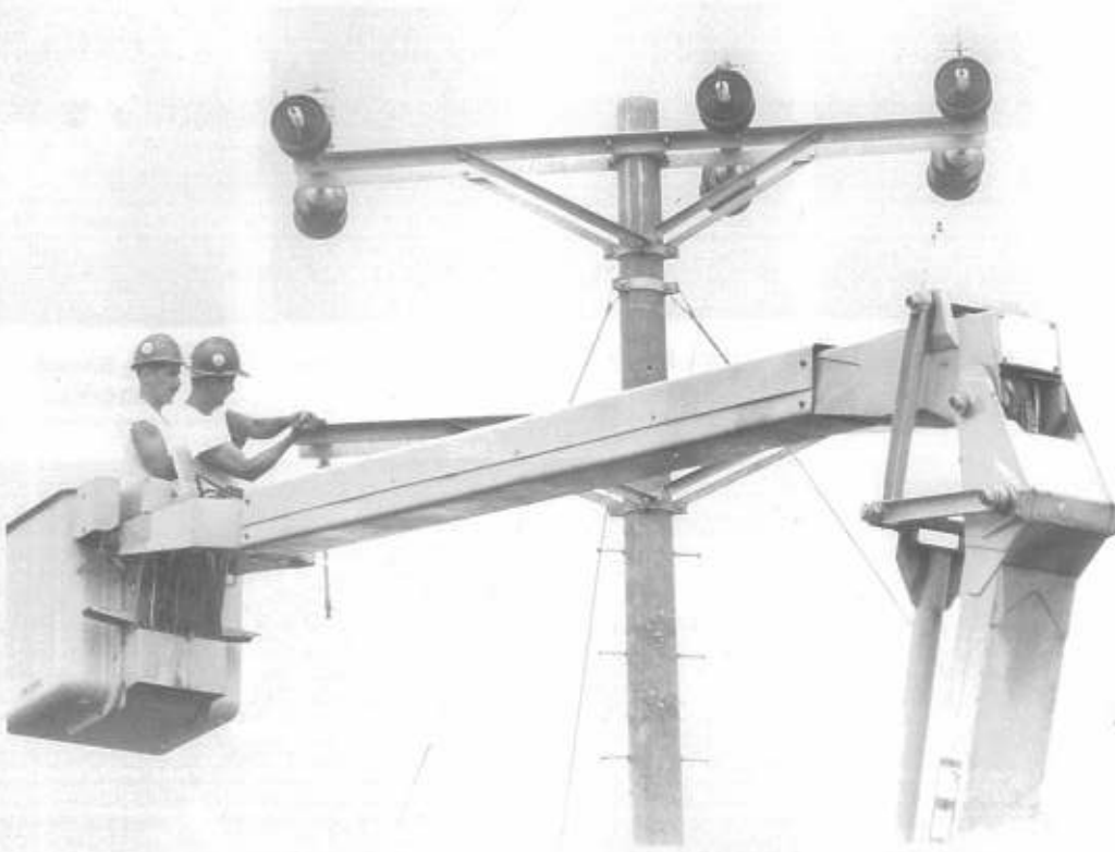
CE3 King and CECN Williams tighten cross arms from boom truck.
