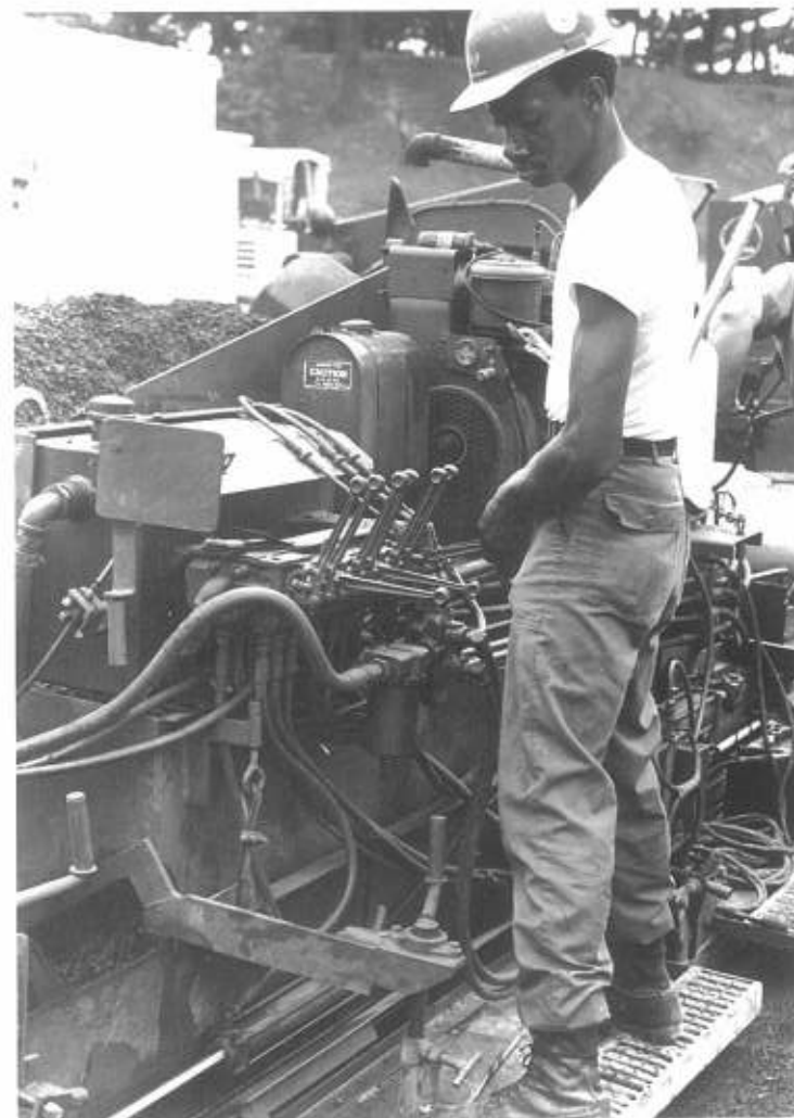
Top — Asphalt crew makes first pass with paver. Above — EO1 Robinson Asphalt crew leader.
