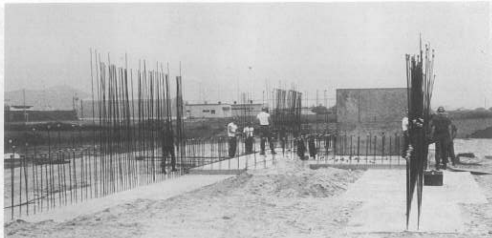
Getting ready to place interior forms at pyrotech project.
