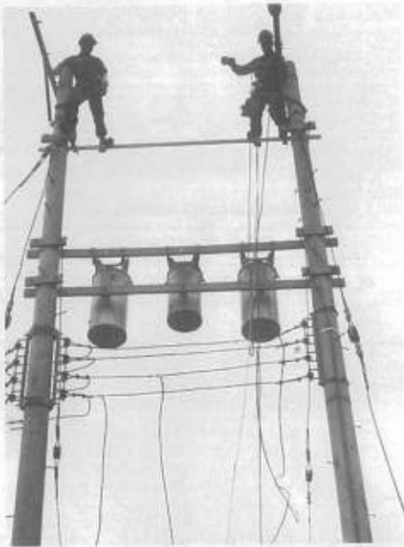
Work goes on around another "H" frame at White Beach.
